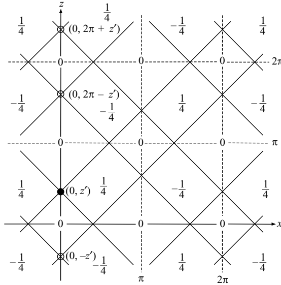
FIGURE 8. The real part of the Green’s function G_b(x, z, z') defined in (19), with a single source at (0, z') and reflecting surfaces along the x -axis and the line z = \pi . In this case the model domain is 0 < z < \pi , and the boundary conditions require an infinite series of vertically displaced mirror sources, alternating between positive and negative sign. This figure corrects figure 3 in Llewellyn Smith & Young (2003), and figure 1 in Robinson (1969).
