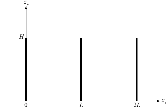
FIGURE 2. The bottom topography, consisting of a periodic series of thin vertical walls, which have height H and are separated by length L .
