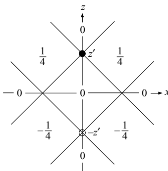
FIGURE 4. The real part of the Green's function G_2(x, z, z') defined in (16), describing the internal wave radiation from a point source at (0, z') with a reflecting surface along the x -axis. Here and in subsequent figures, the solid circles denote sources and the open circles mirror sources, and the region z < 0 , where the negative mirror sources in figures 4–7 are situated, is not part of the model domain.
