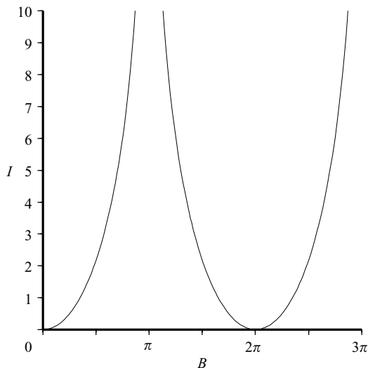
FIGURE 9. Plot of the function I(B) defined in (25) and (36)–(37), showing the radiated power as a function of the dimensionless ridge height B .
