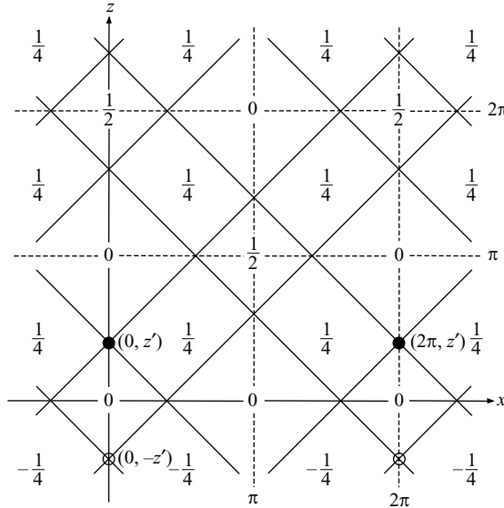
FIGURE 5. The real part of the Green's function G(x, z, z') defined in (17), with sources at (2\pi n, z') and a reflecting surface along the x -axis, for the case 0 < z' < \pi .
