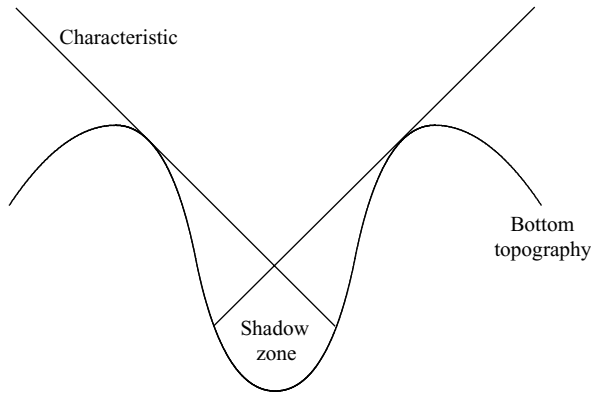
FIGURE 1. Illustration of shadowing. The straight lines are internal wave characteristics that connect to the region above the topography.
