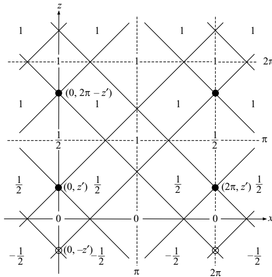
FIGURE 7. The sum G(x, z, z') + G(x, z, 2\pi - z') , where 0 < z' < \pi .
