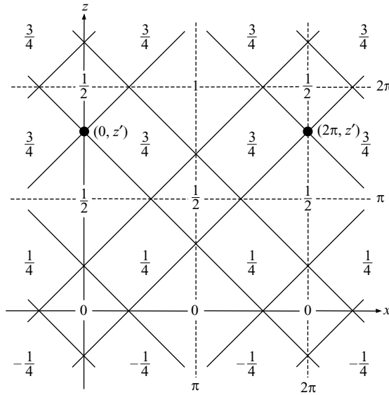
FIGURE 6. The same as figure 5, but for the case \pi < z' < 2\pi .
