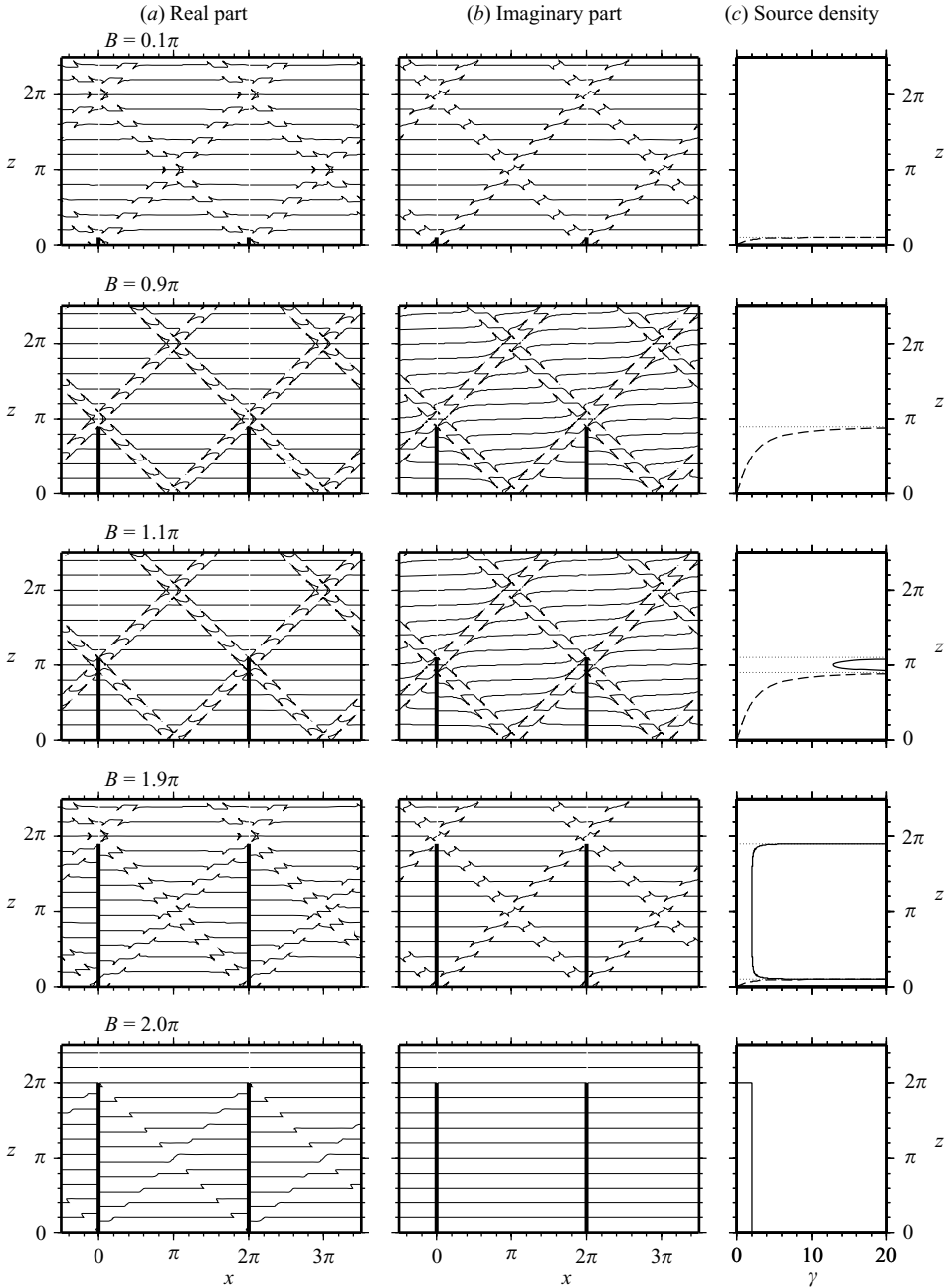
FIGURE 10. Illustration of the wave field and the source density for different values of the dimensionless ridge height B . The contours are curves of constant total density (perturbation plus a linearly stratified background). The real and imaginary parts of the density perturbation has been used in columns (a) and (b), respectively. The source density along the walls is shown in column (c), with the solid curves representing the real part and the dashed curves the imaginary part of \gamma . The dotted lines denote singularities in the source distribution.
