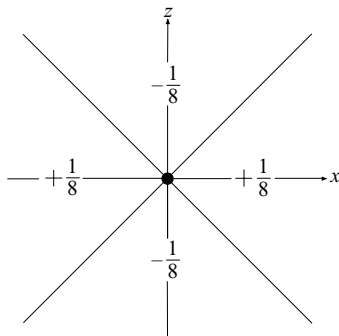
FIGURE 3. The real part of the Green's function G_1 defined in (15), showing the internal wave radiation from a point source (marked by a solid circle) at the origin on an infinite vertical plane.
